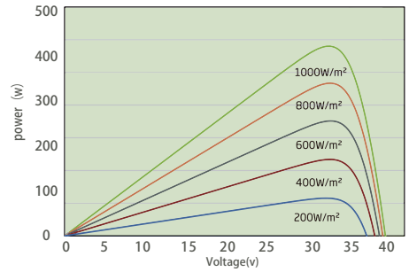
P-V CURVES OF PV MODULE (410w)
