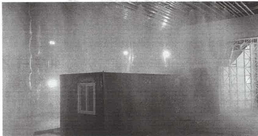
Test-in-process (rainfall intensity: 202mm/h)
