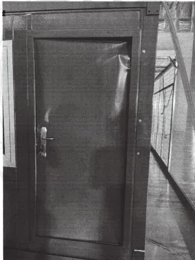
Test-in-process (wind speed: 49.9m/s, level 15)
