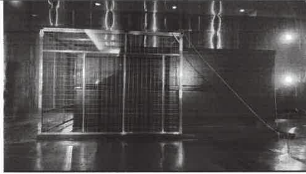
Test-in-process (wind speed: 56.3m/s, level 17)
